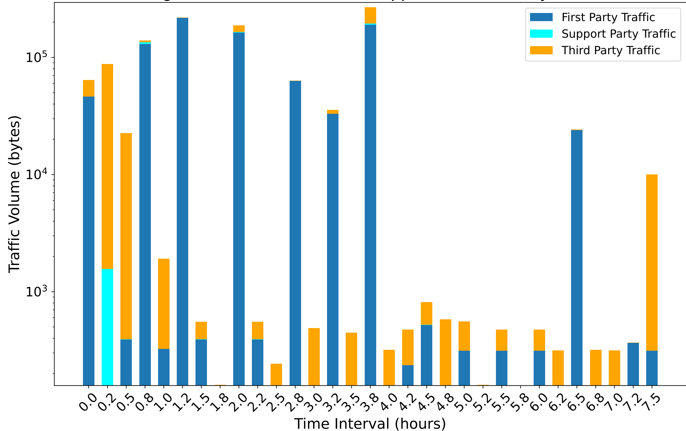
(Log) Traffic Volume: First vs Support vs Third Party Traffic
